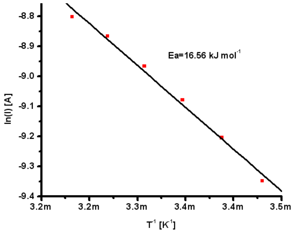
Figure 34 Arrhenius plot
