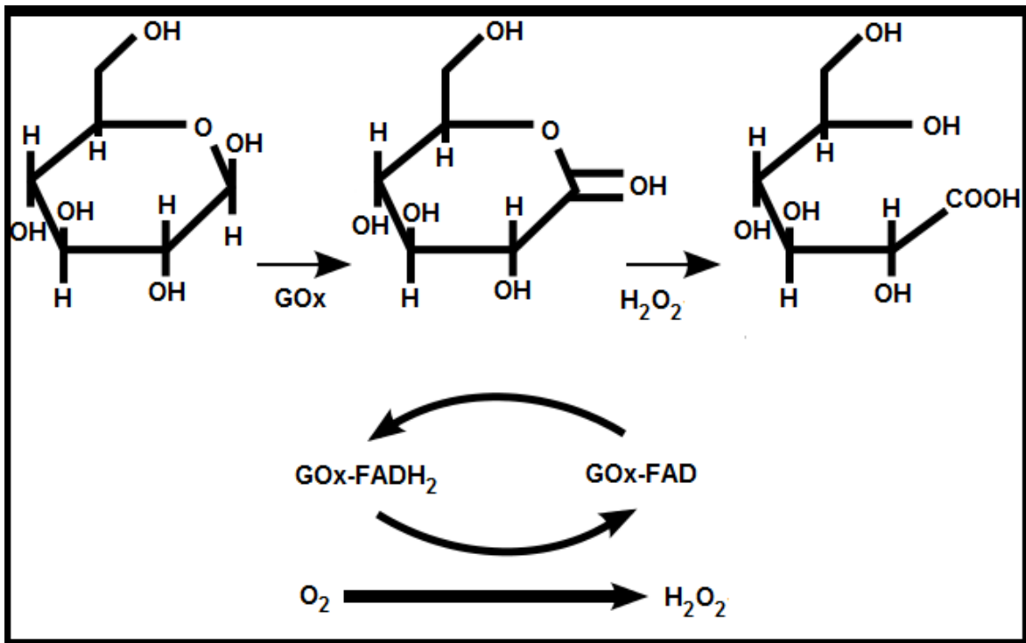
Figure 22 From glucose to gluconic acid
