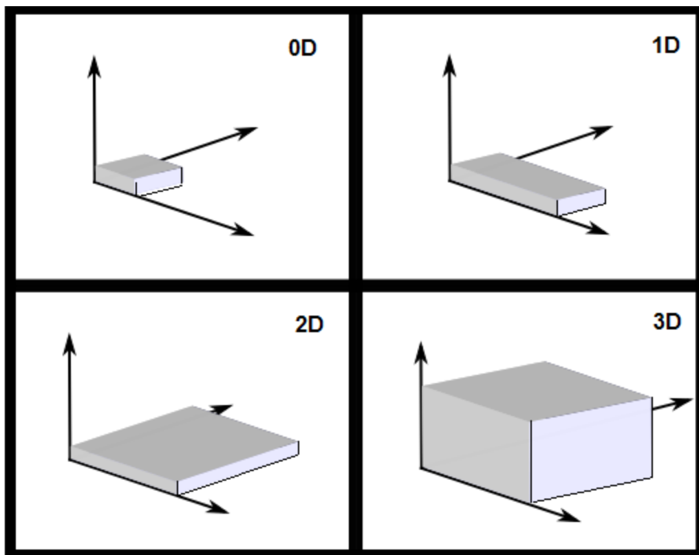
Figure 9 Dimensionality classification
