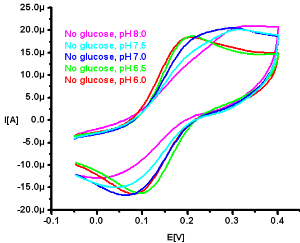
Figure 35 pH studies
